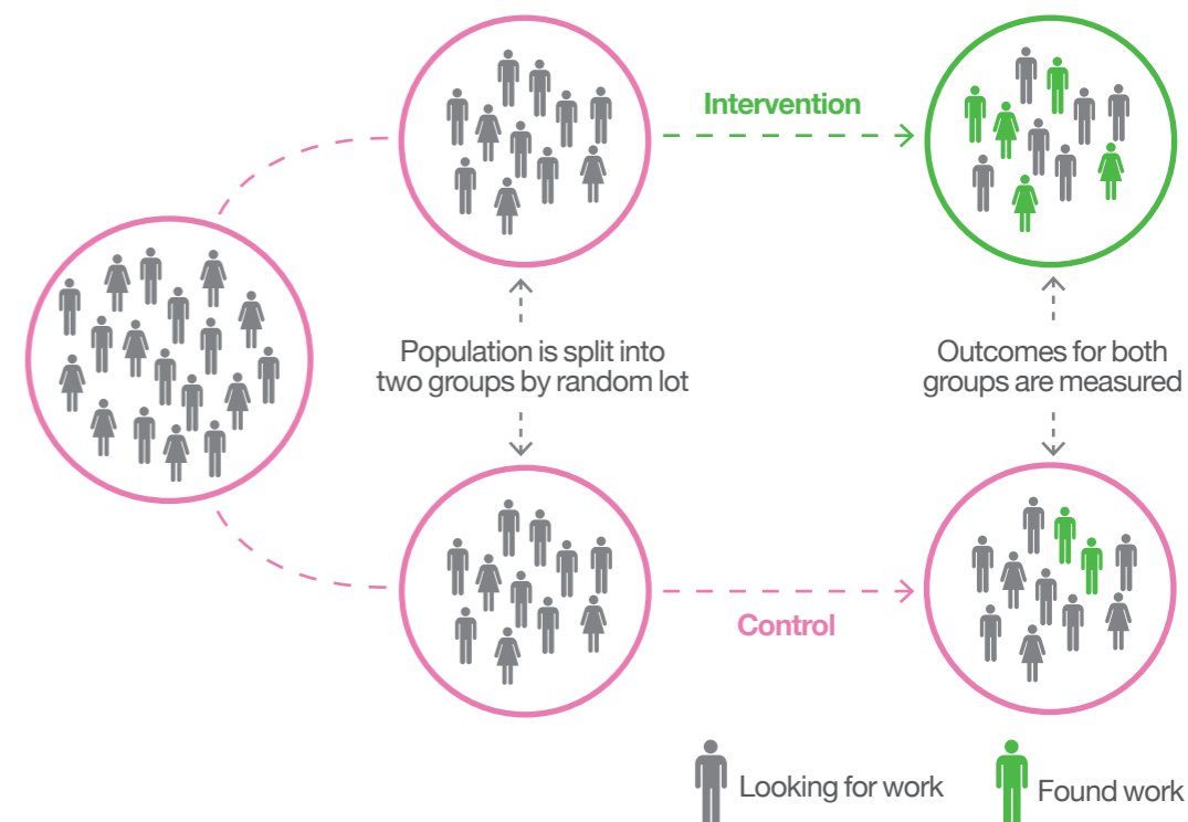
Illustration of a randomised controlled trial (RCT) to test a new ‘back to work’ programme
