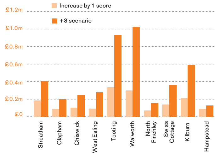
Figure 22: Calculated annual pedestrian user benefits for two improvement scenarios
