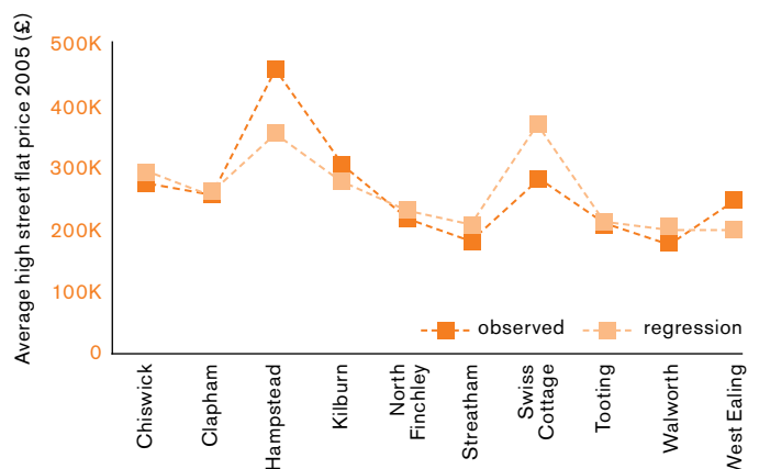
Figure 20: Regression model prices and observed flat prices
